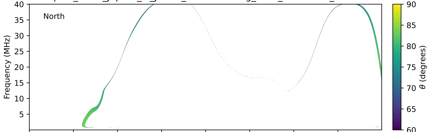
expres_earth_jupiter_io_jrm33_lossc-wid1deg_3kev_20240526_v11.cdf
