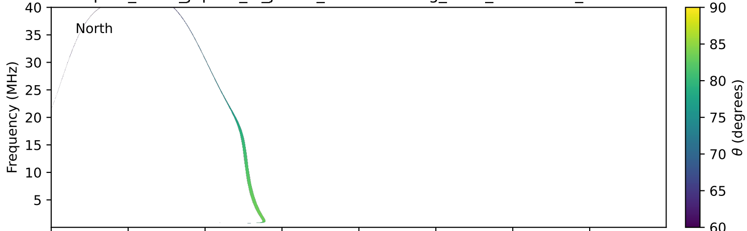
expres_earth_jupiter_io_jrm33_lossc-wid1deg_3kev_20240516_v11.cdf
