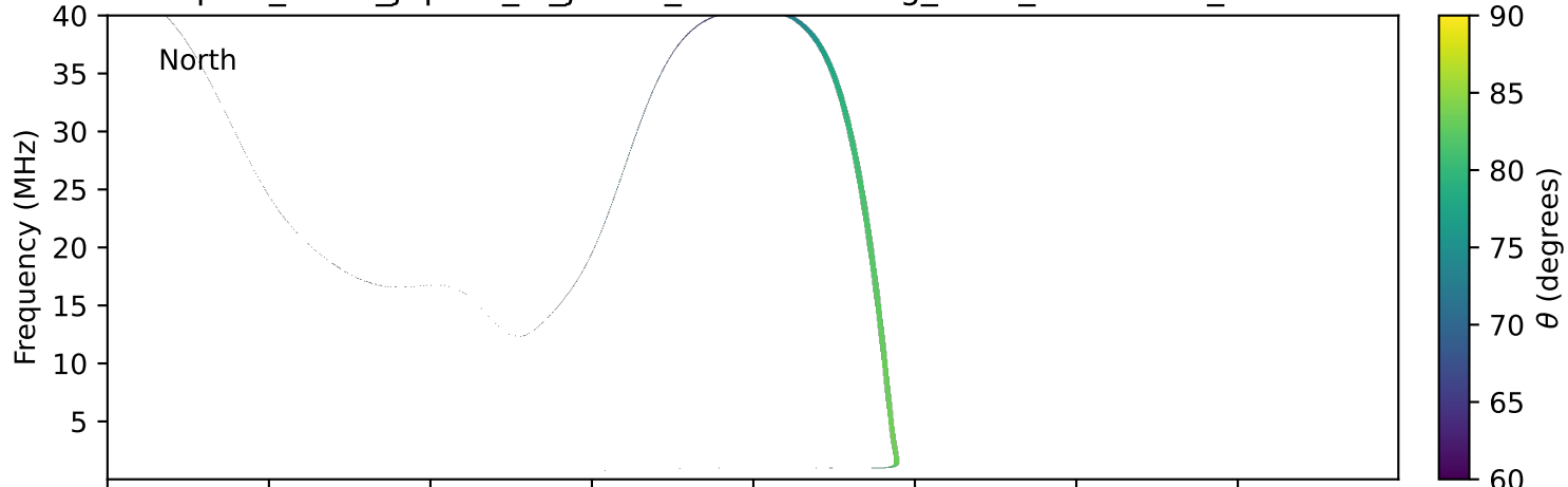
expres_earth_jupiter_io_jrm33_lossc-wid1deg_3kev_20240514_v11.cdf
