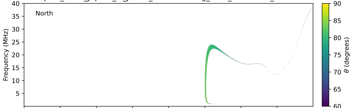
expres_earth_jupiter_io_jrm33_lossc-wid1deg_3kev_20240508_v11.cdf
