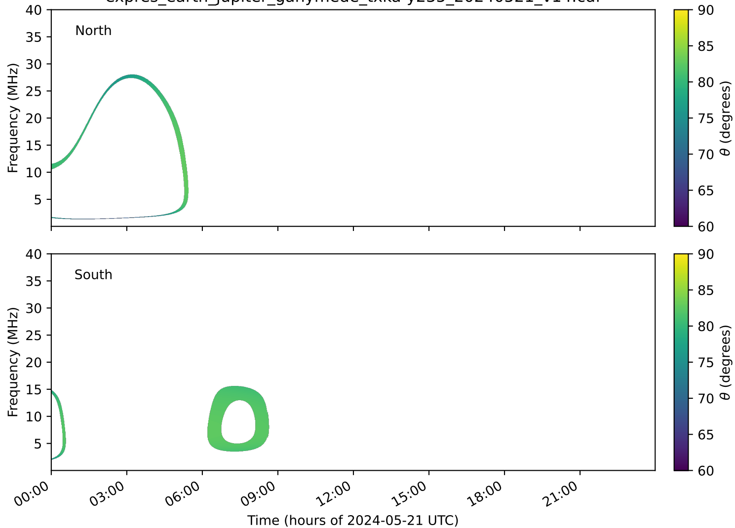
expres_earth_jupiter_ganymede_txka-y235_20240521_v14.cdf
