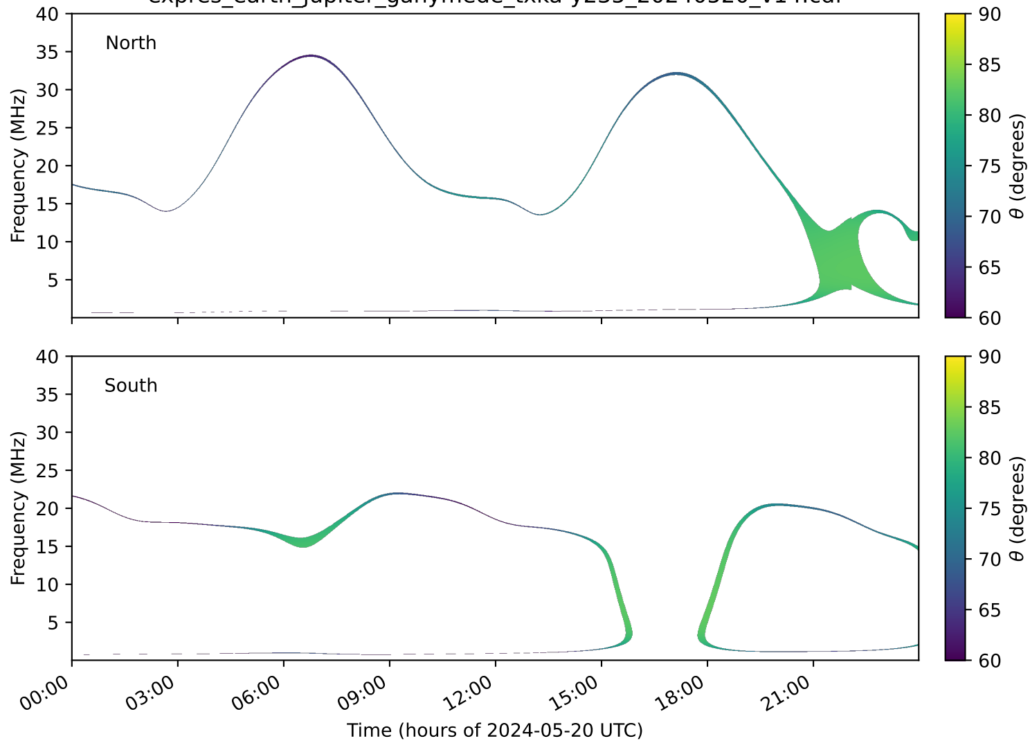
expres_earth_jupiter_ganymede_txka-y235_20240520_v14.cdf
