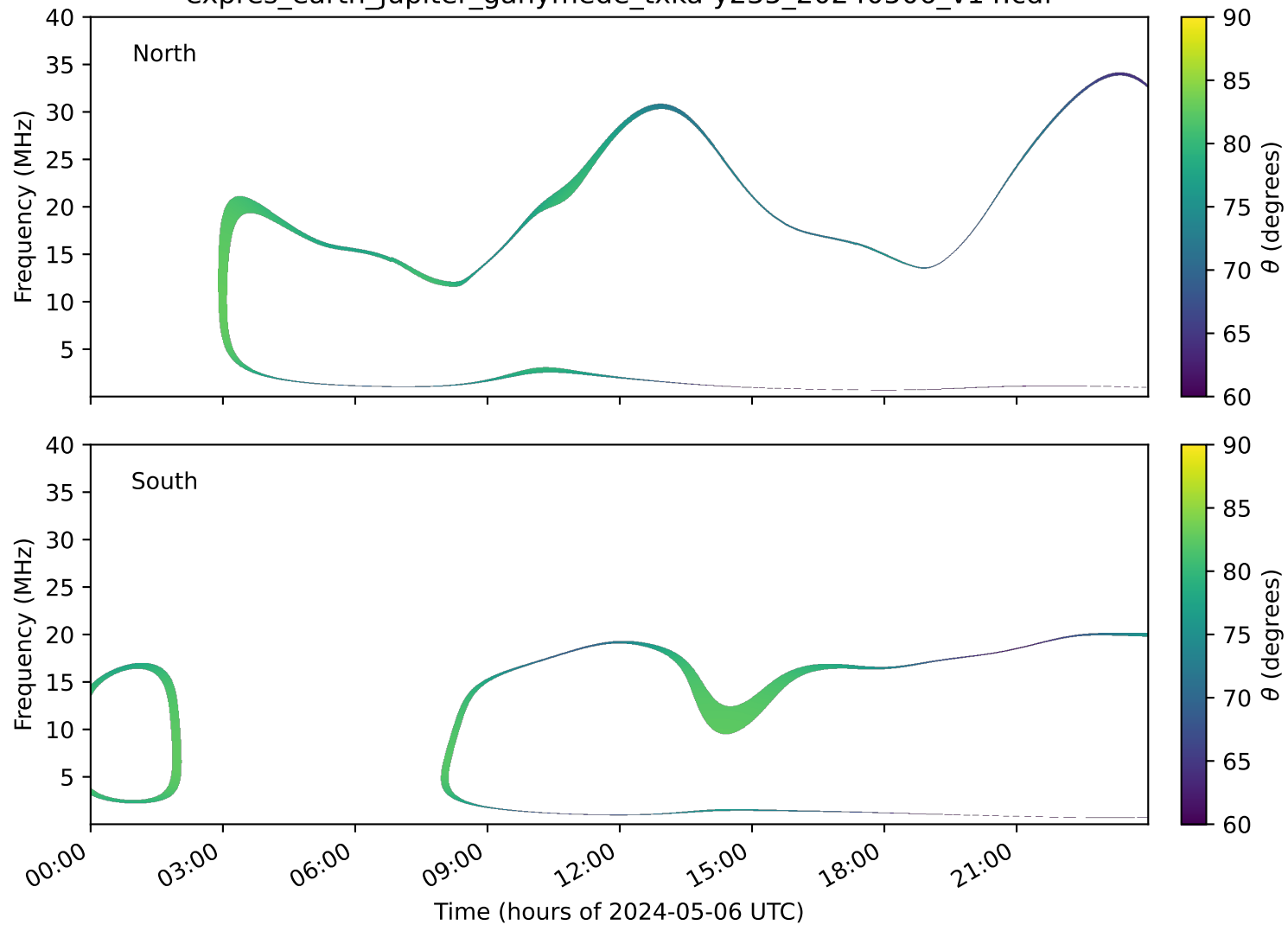
expres_earth_jupiter_ganymede_txka-y235_20240506_v14.cdf
