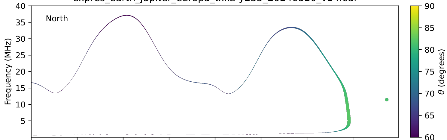
expres_earth_jupiter_europa_txka-y235_20240520_v14.cdf
