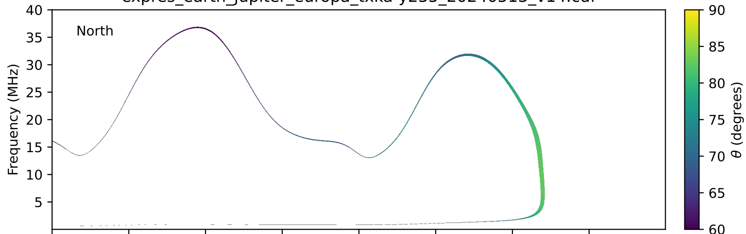
expres_earth_jupiter_europa_txka-y235_20240513_v14.cdf
