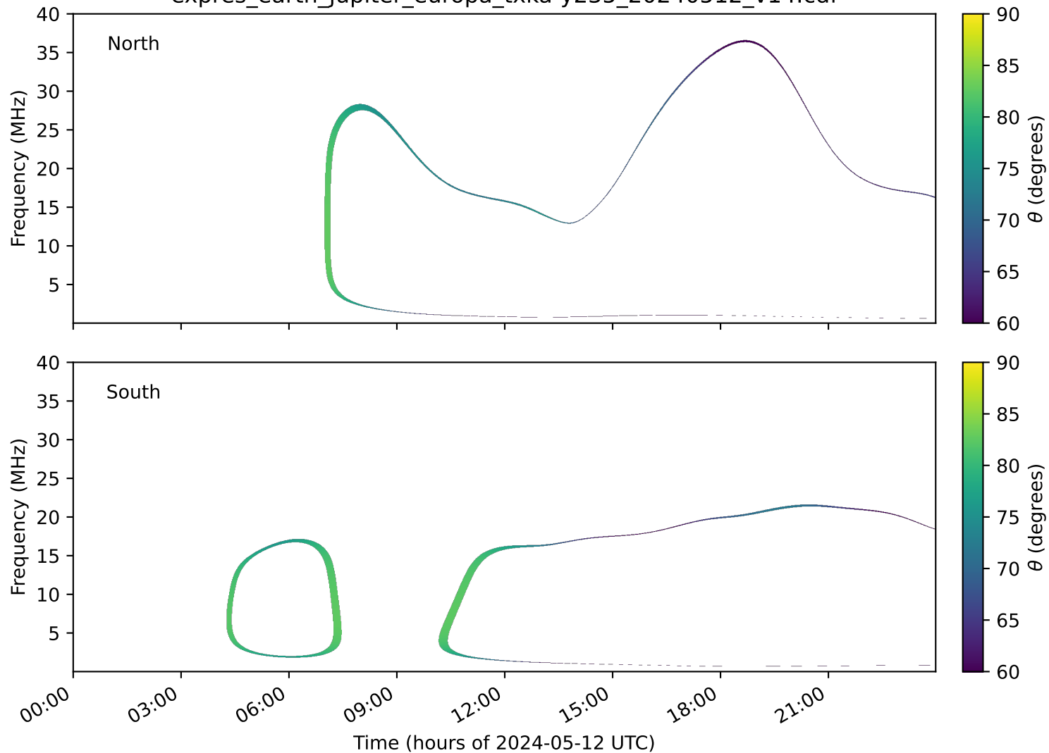
expres_earth_jupiter_europa_txka-y235_20240512_v14.cdf
