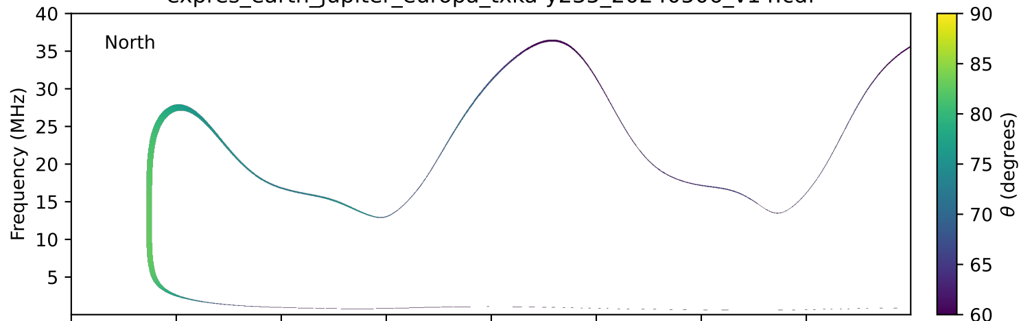
expres_earth_jupiter_europa_txka-y235_20240506_v14.cdf
