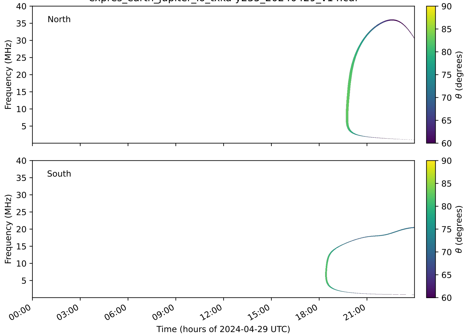
expres_earth_jupiter_io_txka-y235_20240429_v14.cdf
