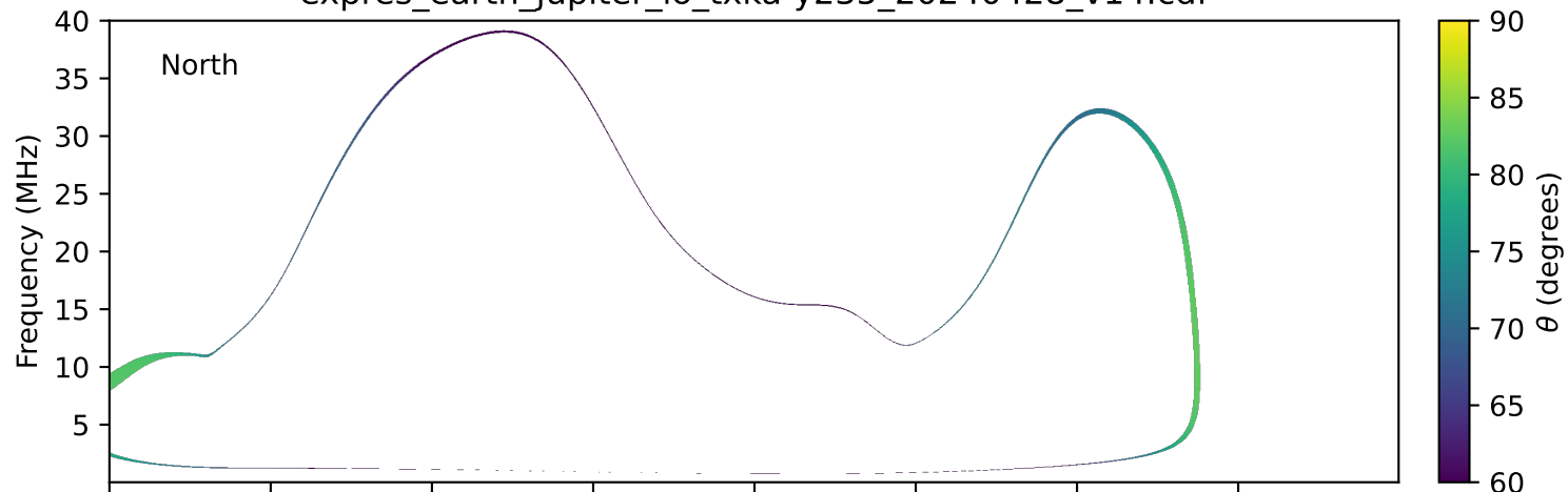
expres_earth_jupiter_io_txka-y235_20240428_v14.cdf
