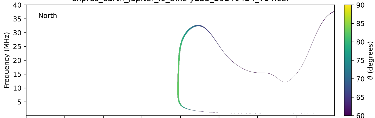
expres_earth_jupiter_io_txka-y235_20240424_v14.cdf
