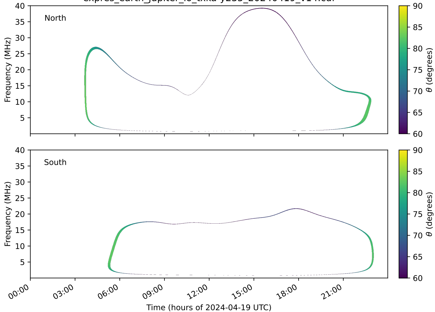
expres_earth_jupiter_io_txka-y235_20240419_v14.cdf
