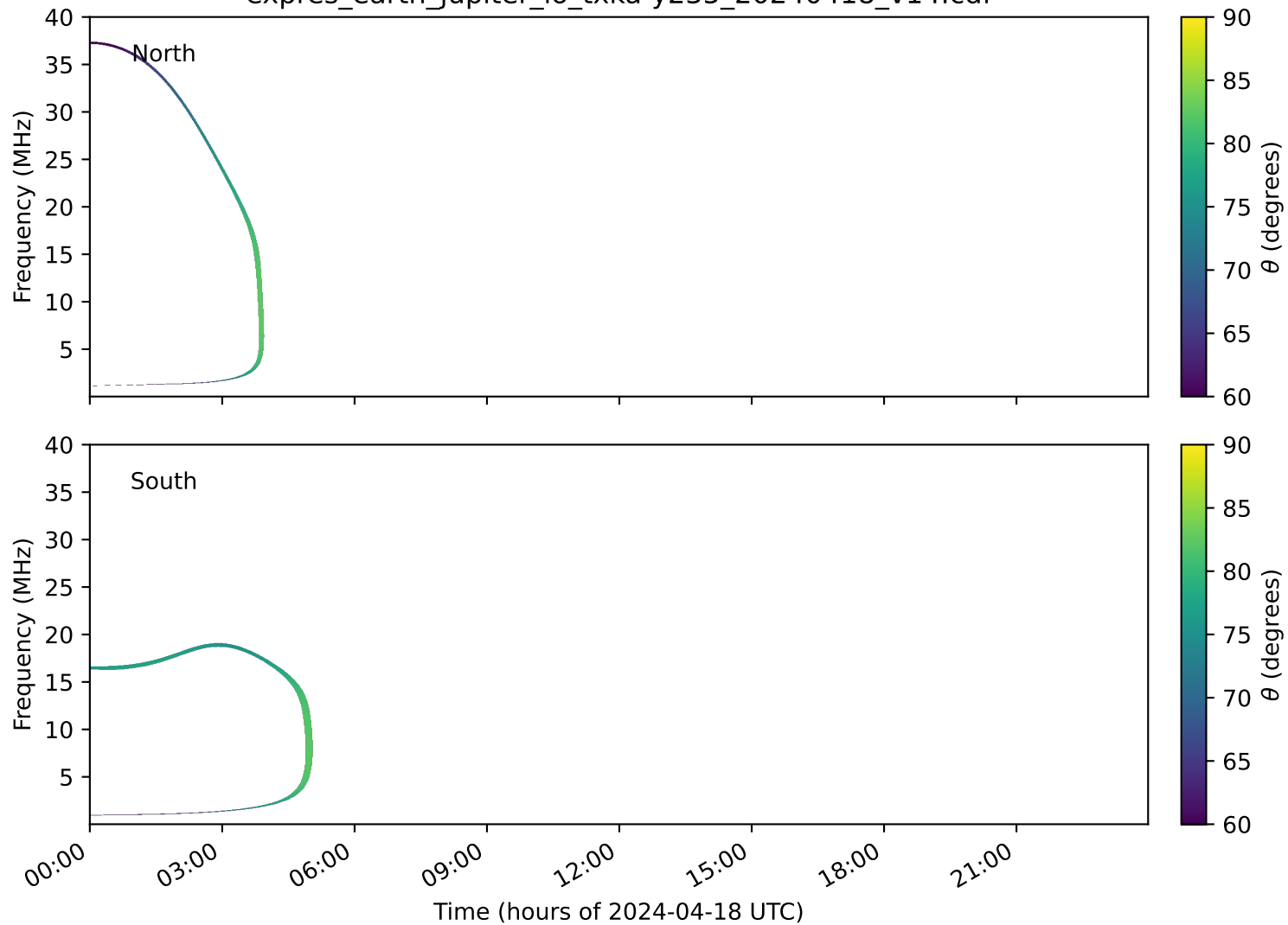
expres_earth_jupiter_io_txka-y235_20240418_v14.cdf
