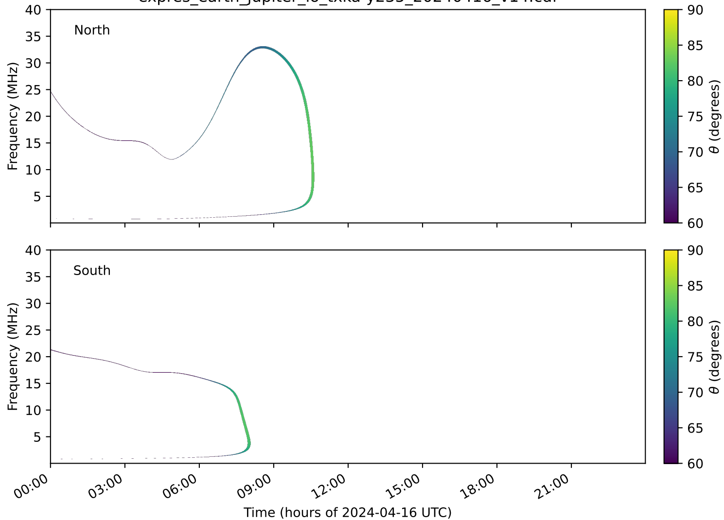
expres_earth_jupiter_io_txka-y235_20240416_v14.cdf
