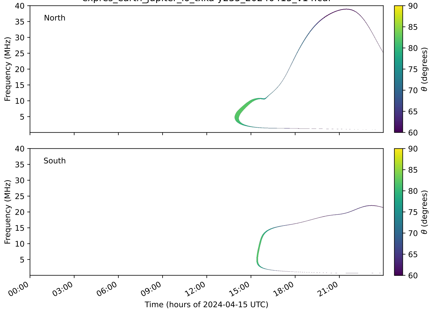
expres_earth_jupiter_io_txka-y235_20240415_v14.cdf
