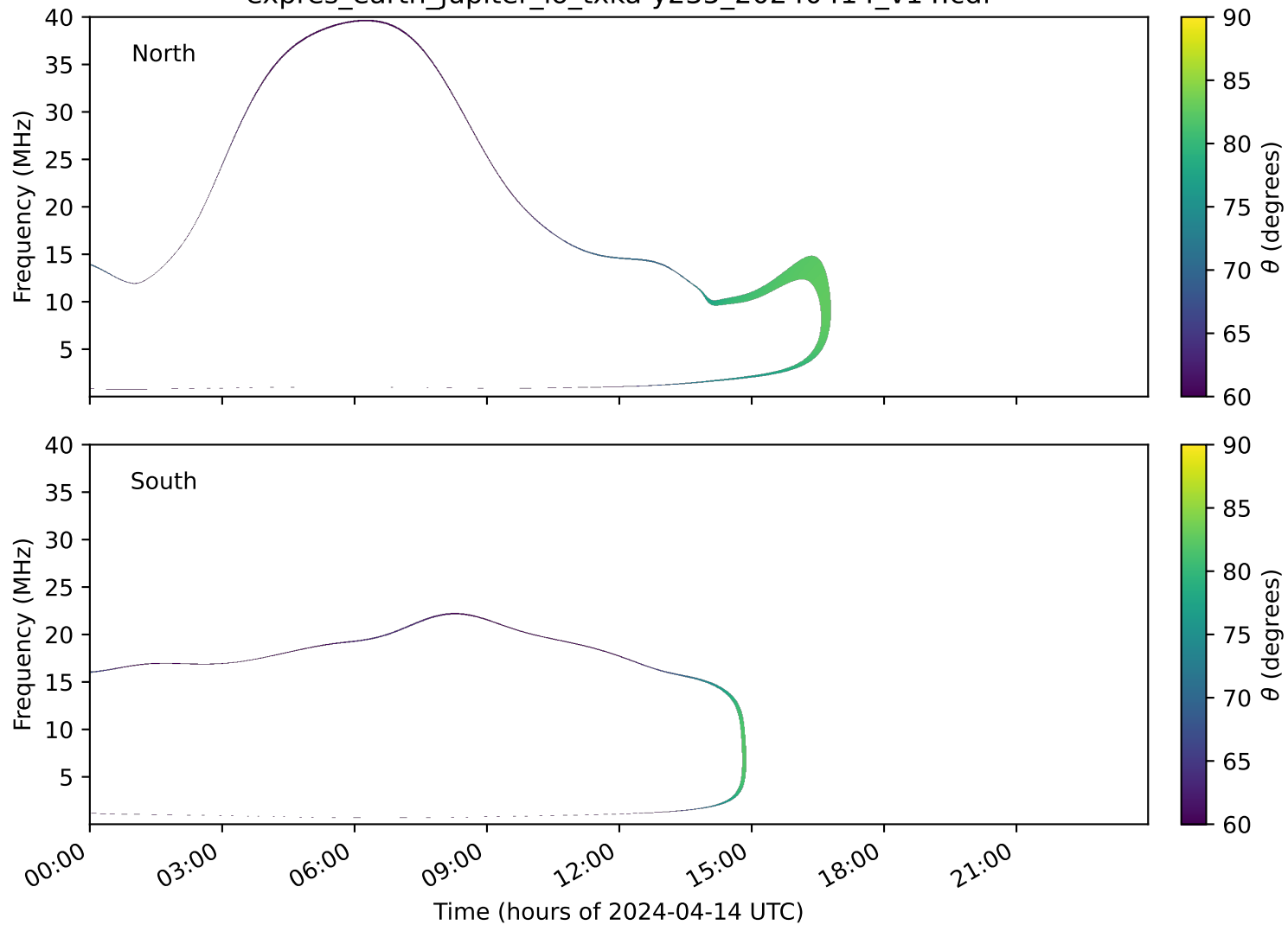
expres_earth_jupiter_io_txka-y235_20240414_v14.cdf
