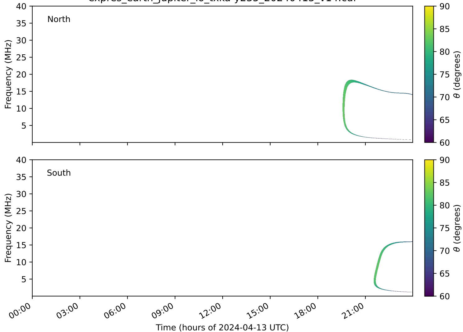
expres_earth_jupiter_io_txka-y235_20240413_v14.cdf
