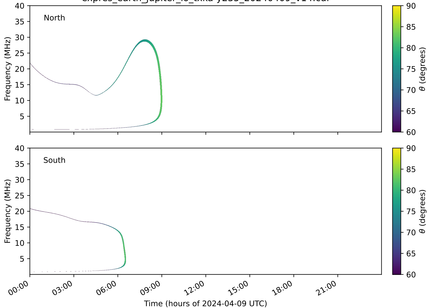
expres_earth_jupiter_io_txka-y235_20240409_v14.cdf
