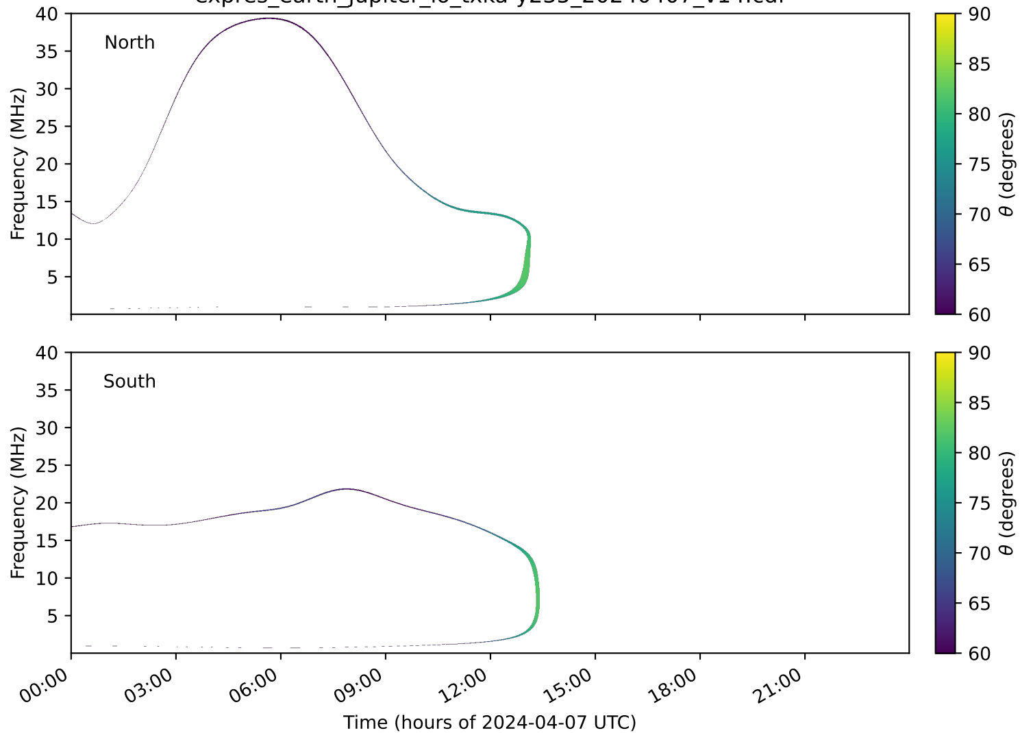
expres_earth_jupiter_io_txka-y235_20240407_v14.cdf
