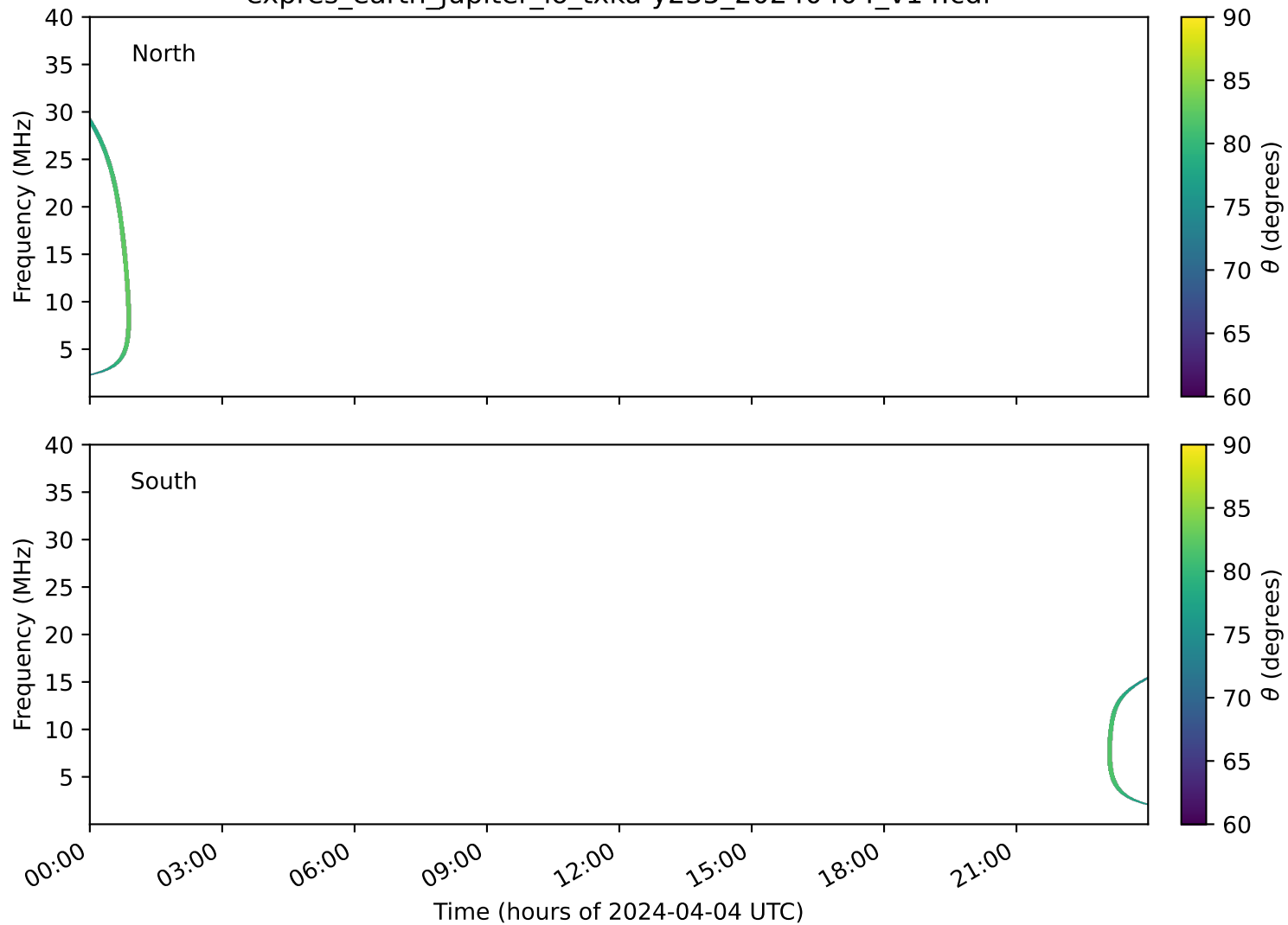
expres_earth_jupiter_io_txka-y235_20240404_v14.cdf
