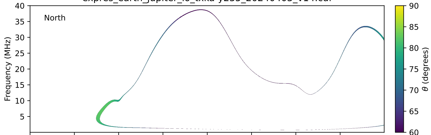
expres_earth_jupiter_io_txka-y235_20240403_v14.cdf
