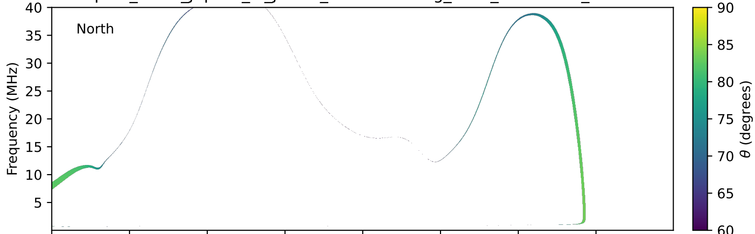
expres_earth_jupiter_io_jrm33_lossc-wid1deg_3kev_20240428_v11.cdf
