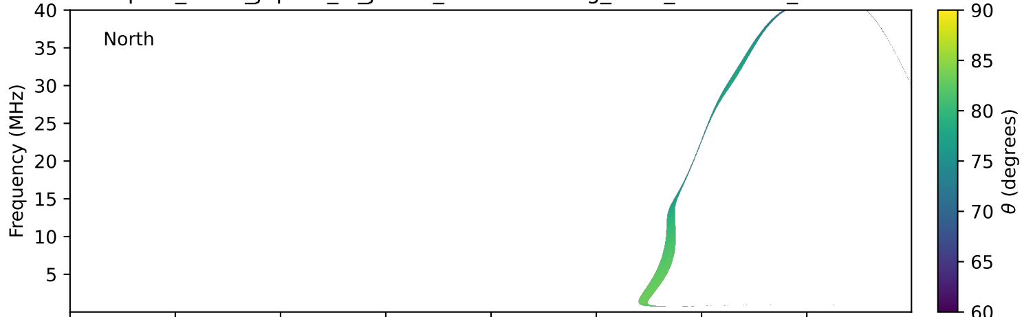
expres_earth_jupiter_io_jrm33_lossc-wid1deg_3kev_20240422_v11.cdf
