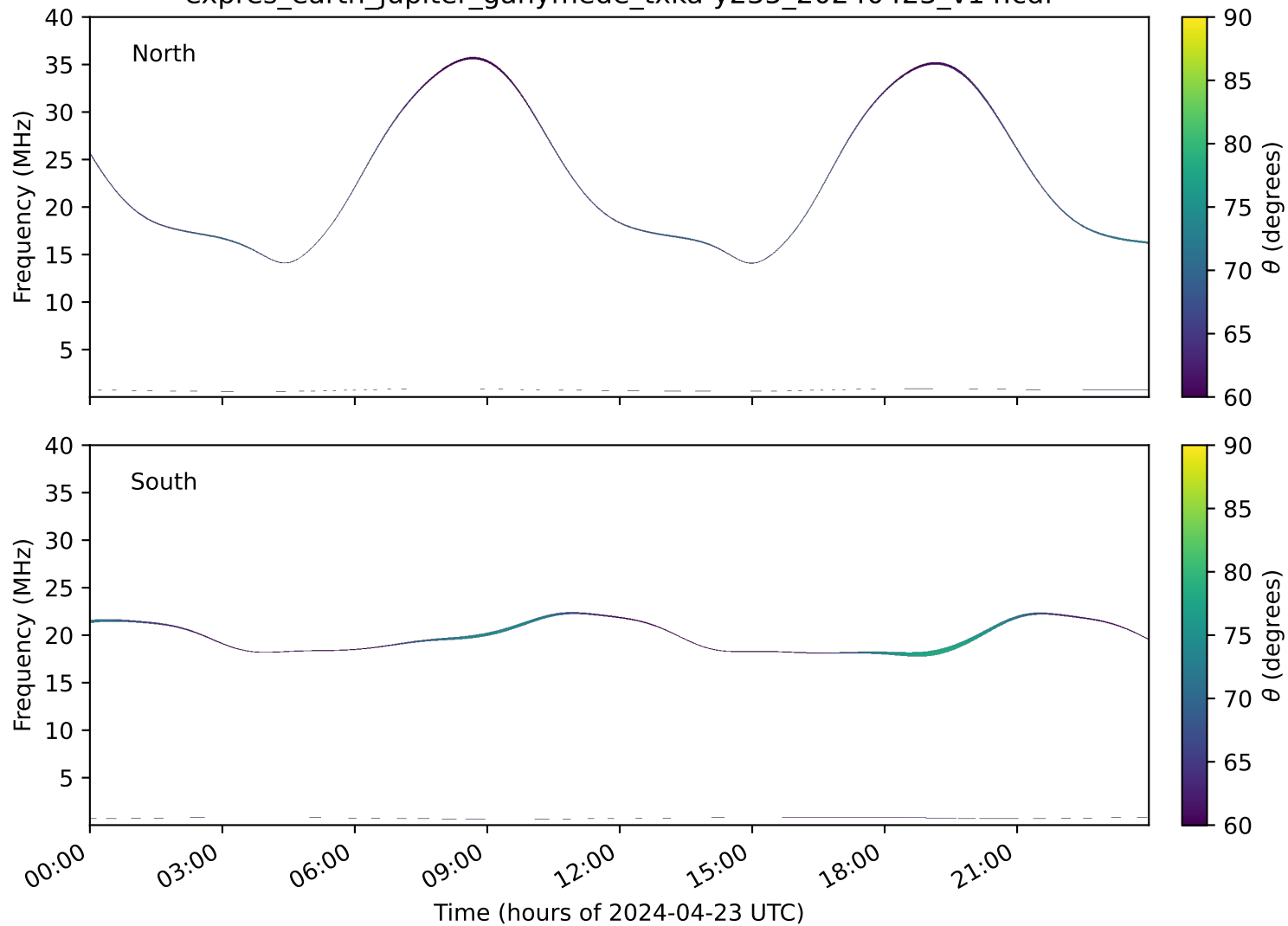
expres_earth_jupiter_ganymede_txka-y235_20240423_v14.cdf
