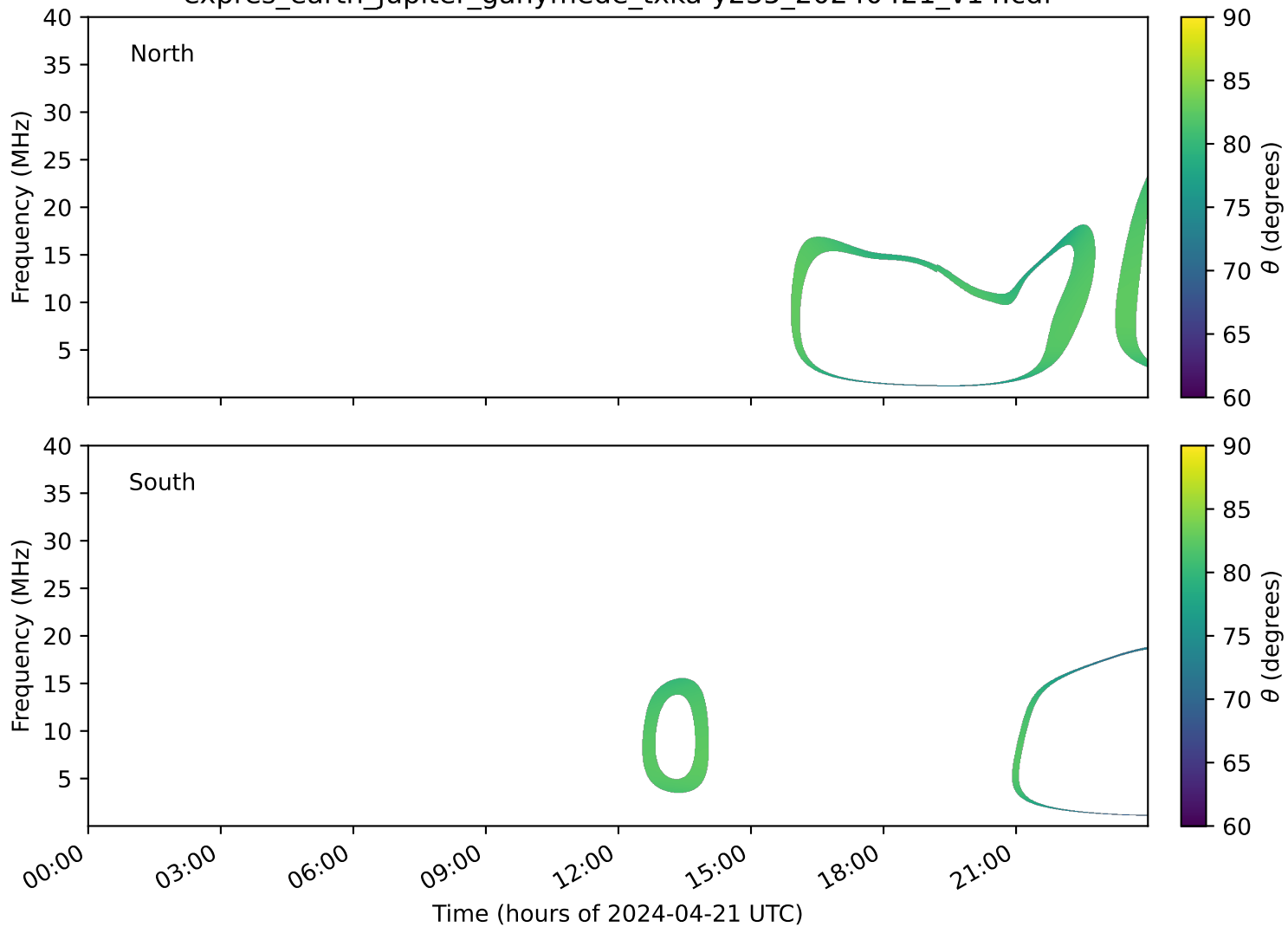
expres_earth_jupiter_ganymede_txka-y235_20240421_v14.cdf
