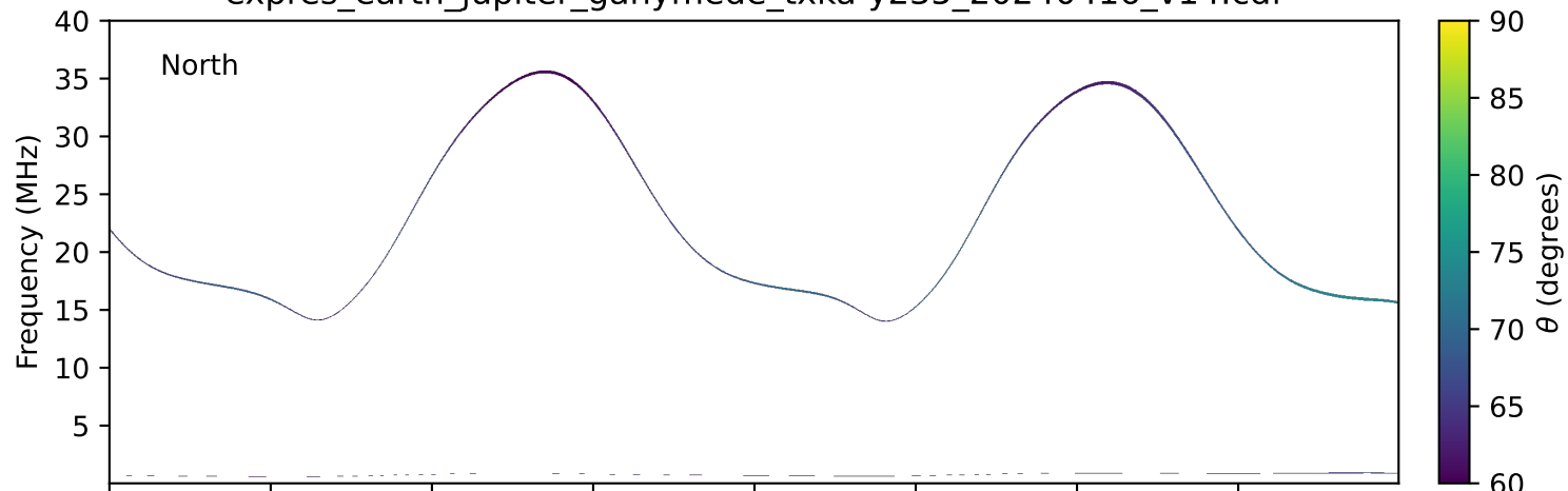
expres_earth_jupiter_ganymede_txka-y235_20240416_v14.cdf
