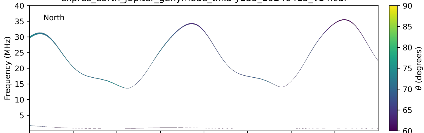
expres_earth_jupiter_ganymede_txka-y235_20240415_v14.cdf
