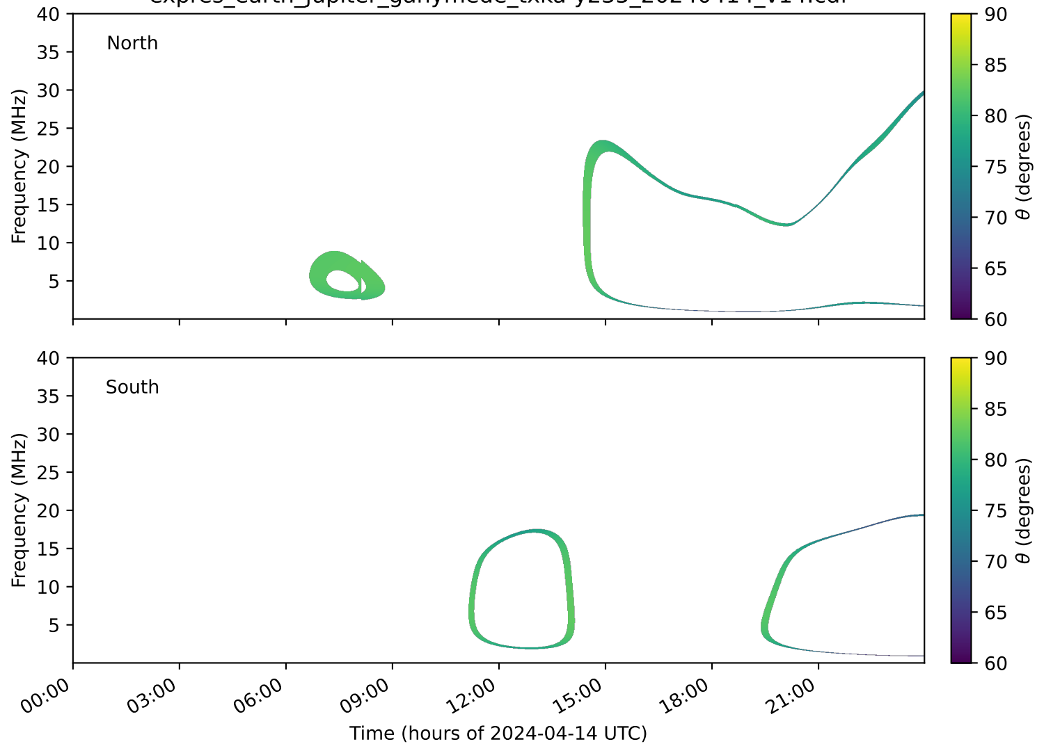
expres_earth_jupiter_ganymede_txka-y235_20240414_v14.cdf
