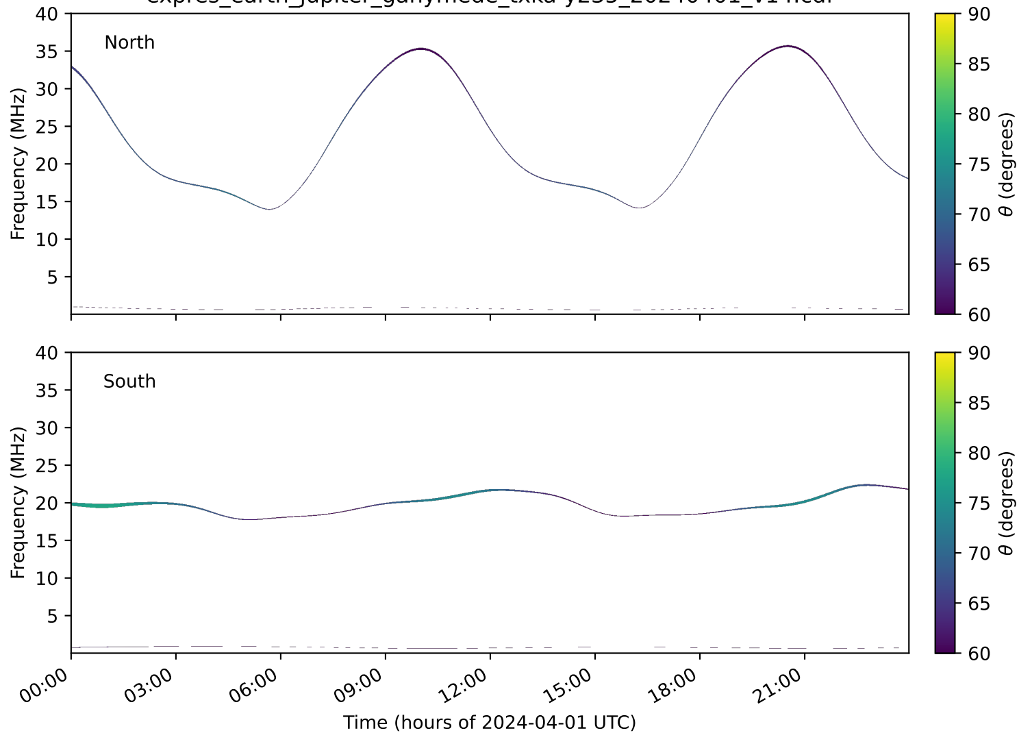
expres_earth_jupiter_ganymede_txka-y235_20240401_v14.cdf
