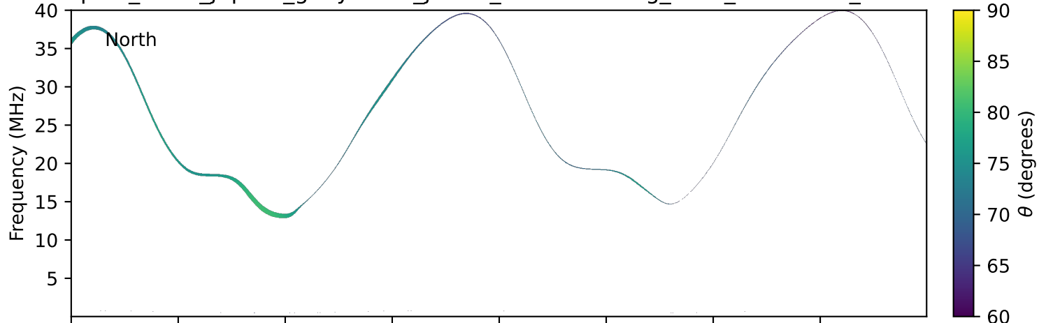
expres_earth_jupiter_ganymede_jrm33_lossc-wid1deg_3kev_20240415_v11.cdf
