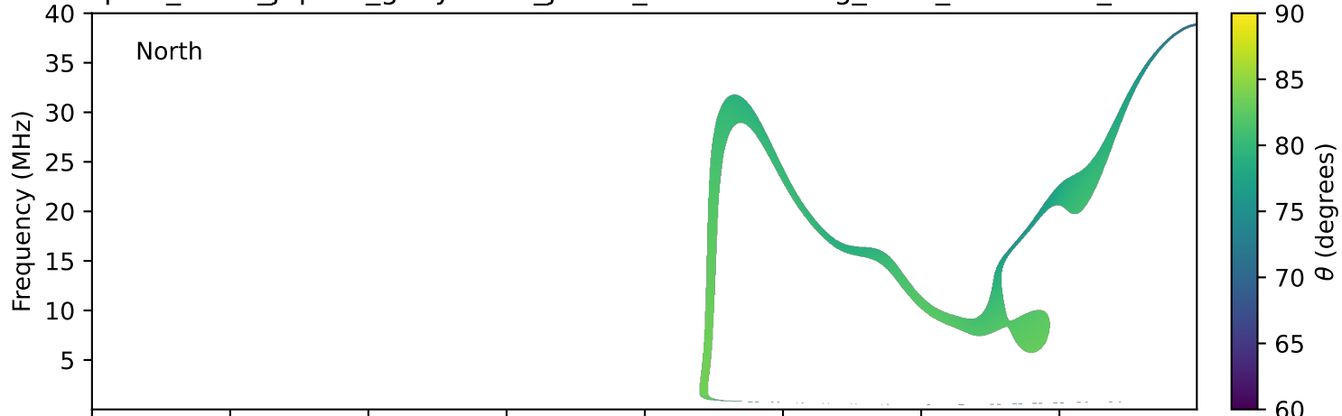
expres_earth_jupiter_ganymede_jrm33_lossc-wid1deg_3kev_20240407_v11.cdf
