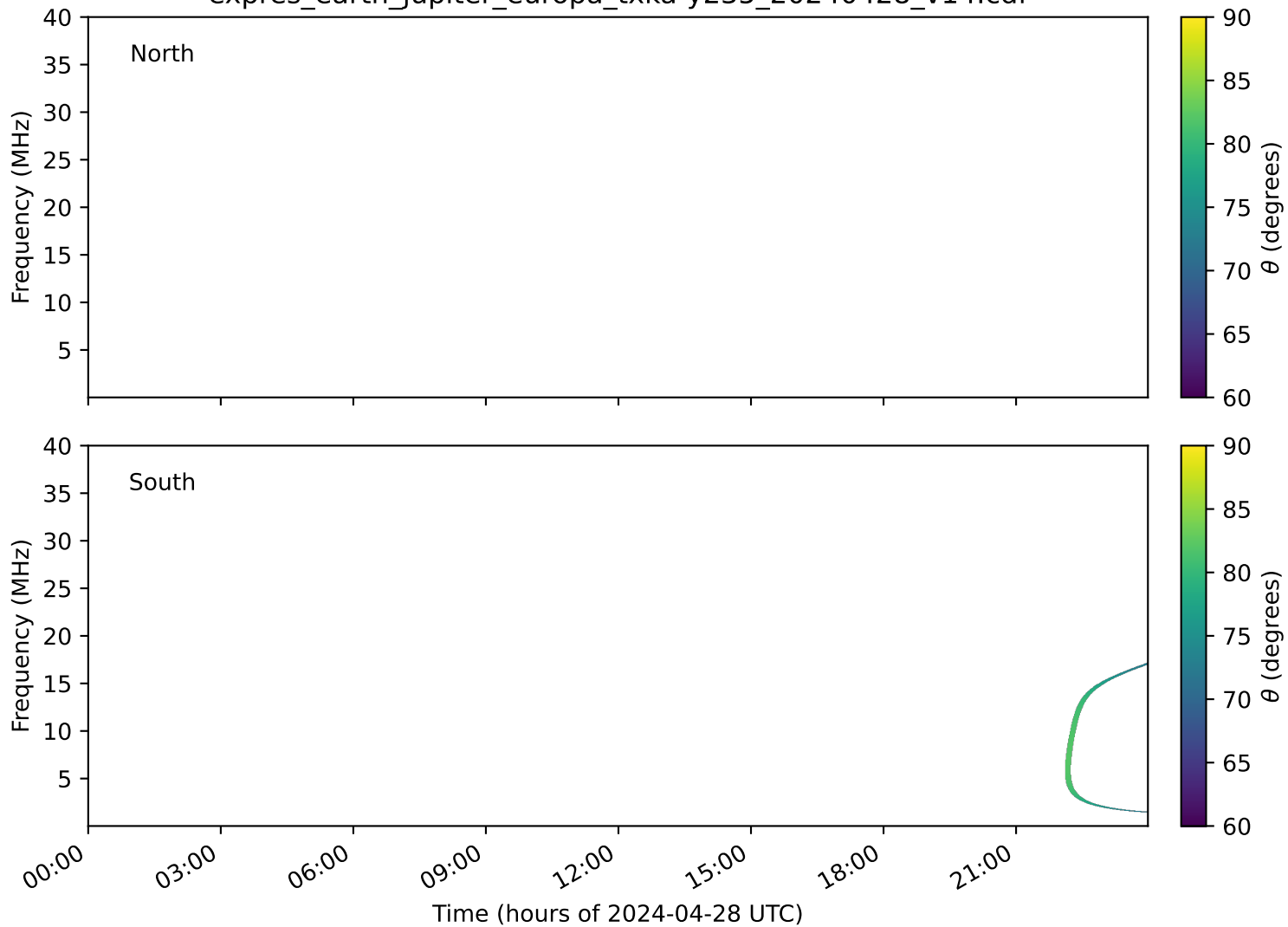
expres_earth_jupiter_europa_txka-y235_20240428_v14.cdf
