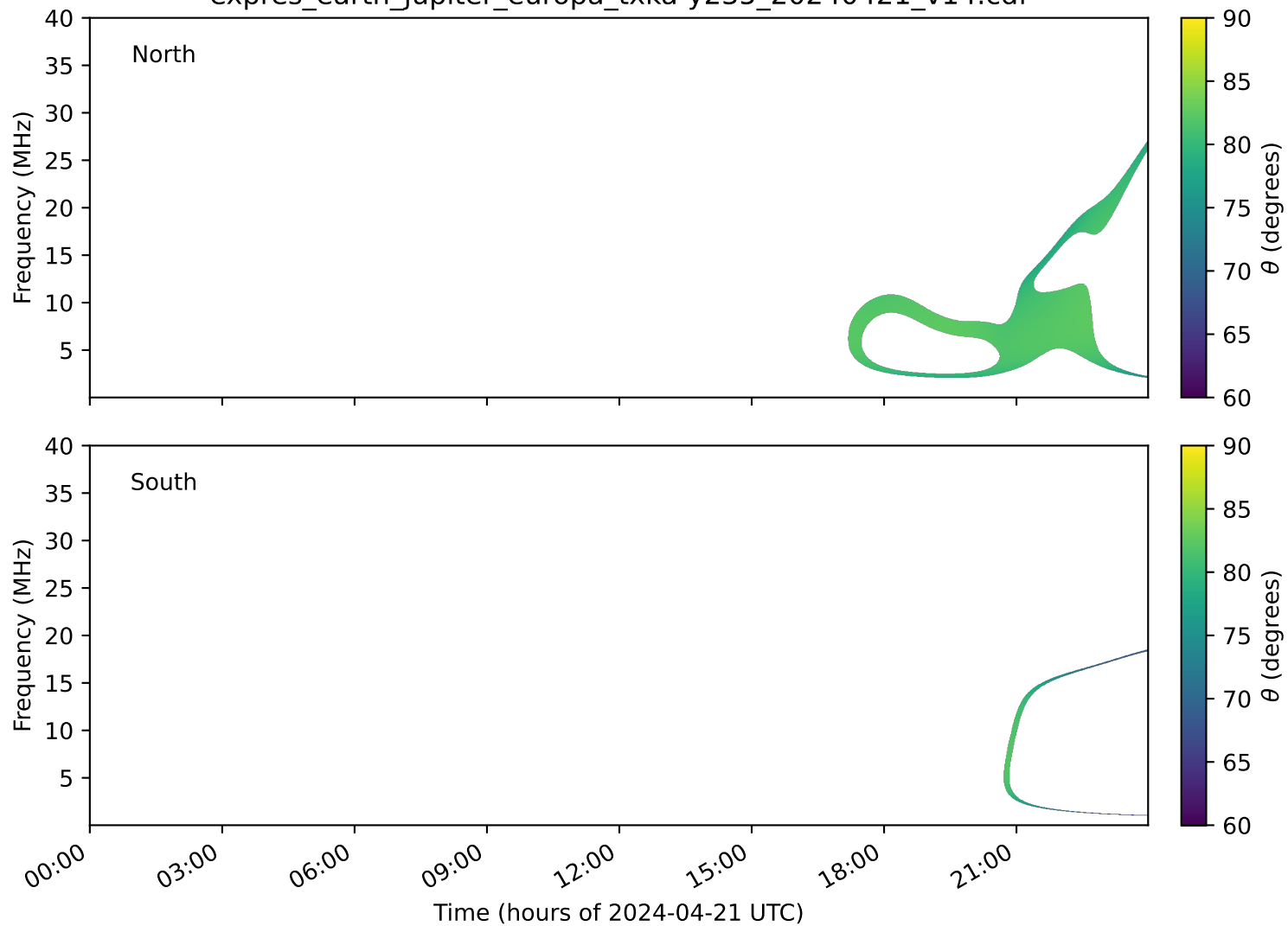
expres_earth_jupiter_europa_txka-y235_20240421_v14.cdf
