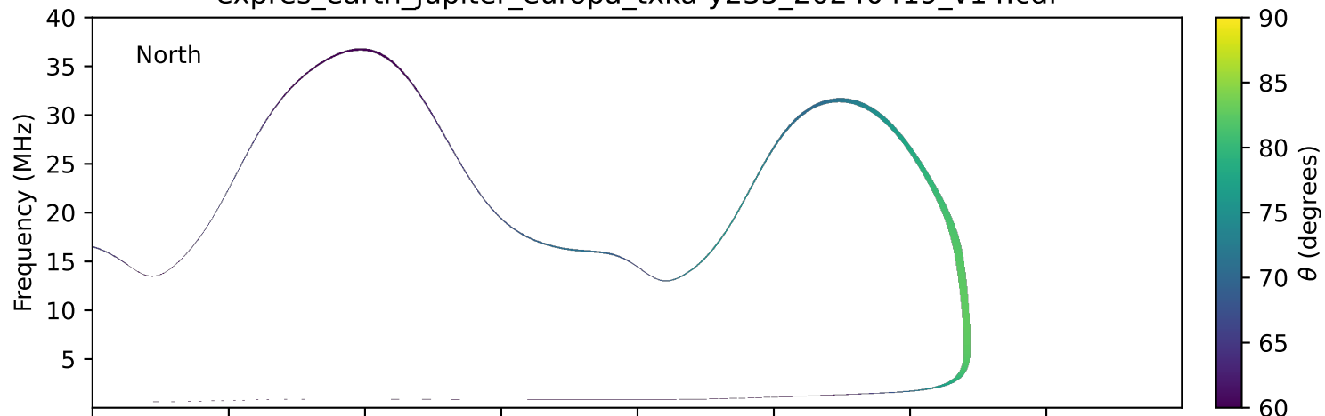
expres_earth_jupiter_europa_txka-y235_20240419_v14.cdf
