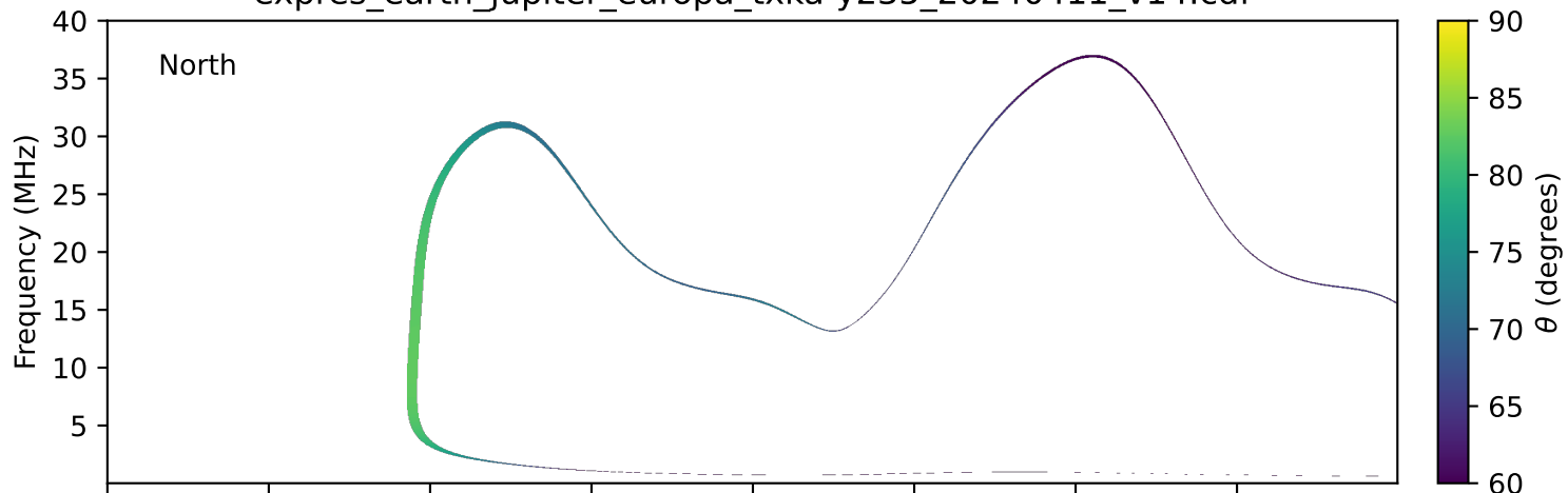
expres_earth_jupiter_europa_txka-y235_20240411_v14.cdf
