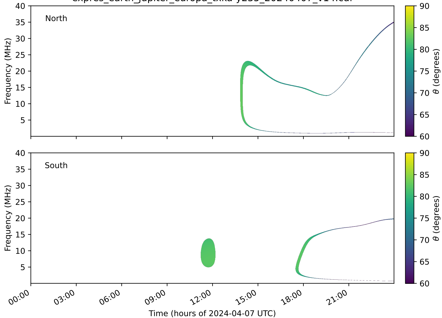
expres_earth_jupiter_europa_txka-y235_20240407_v14.cdf
