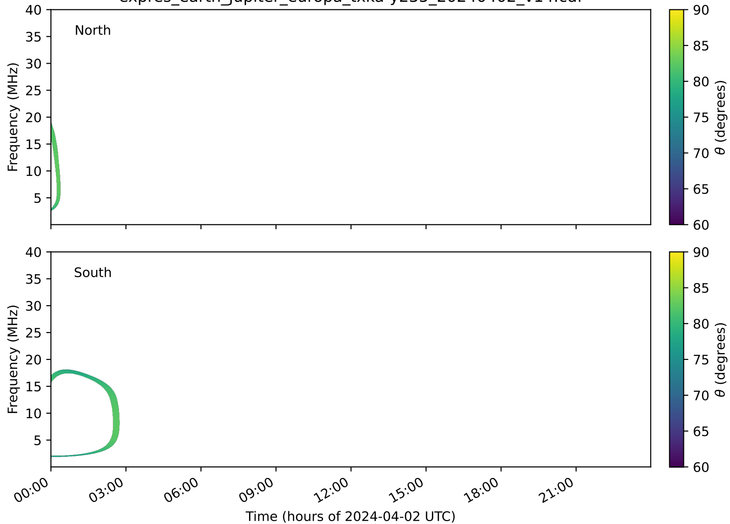
expres_earth_jupiter_europa_txka-y235_20240402_v14.cdf
