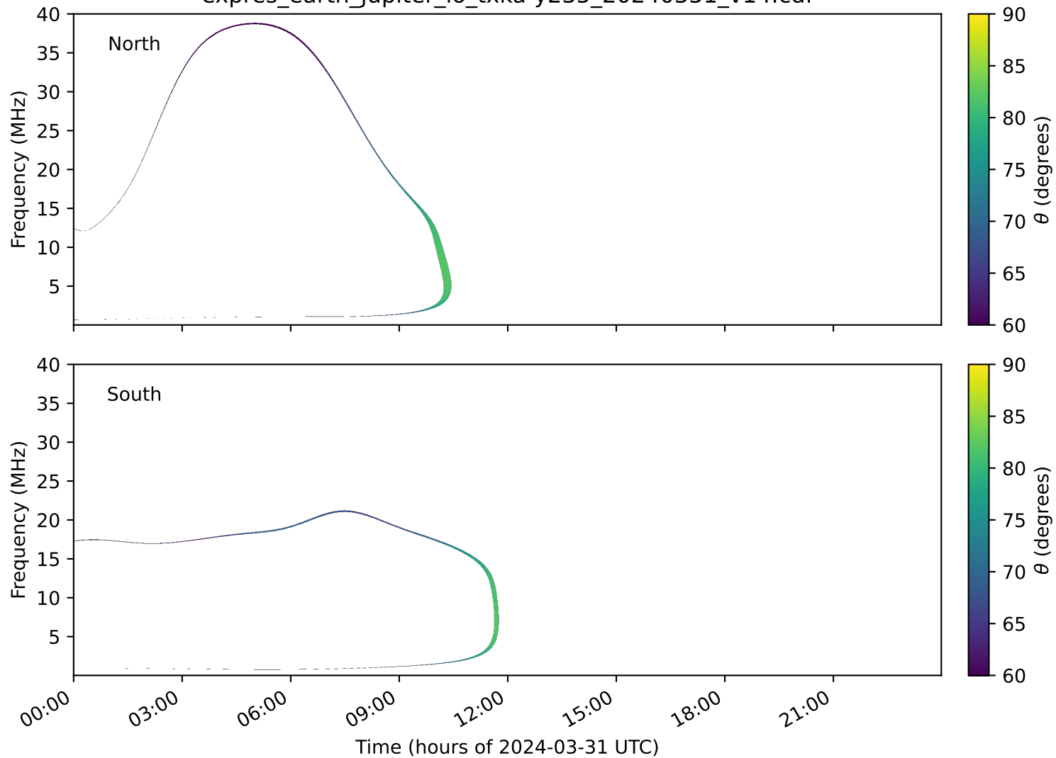
expres_earth_jupiter_io_txka-y235_20240331_v14.cdf
