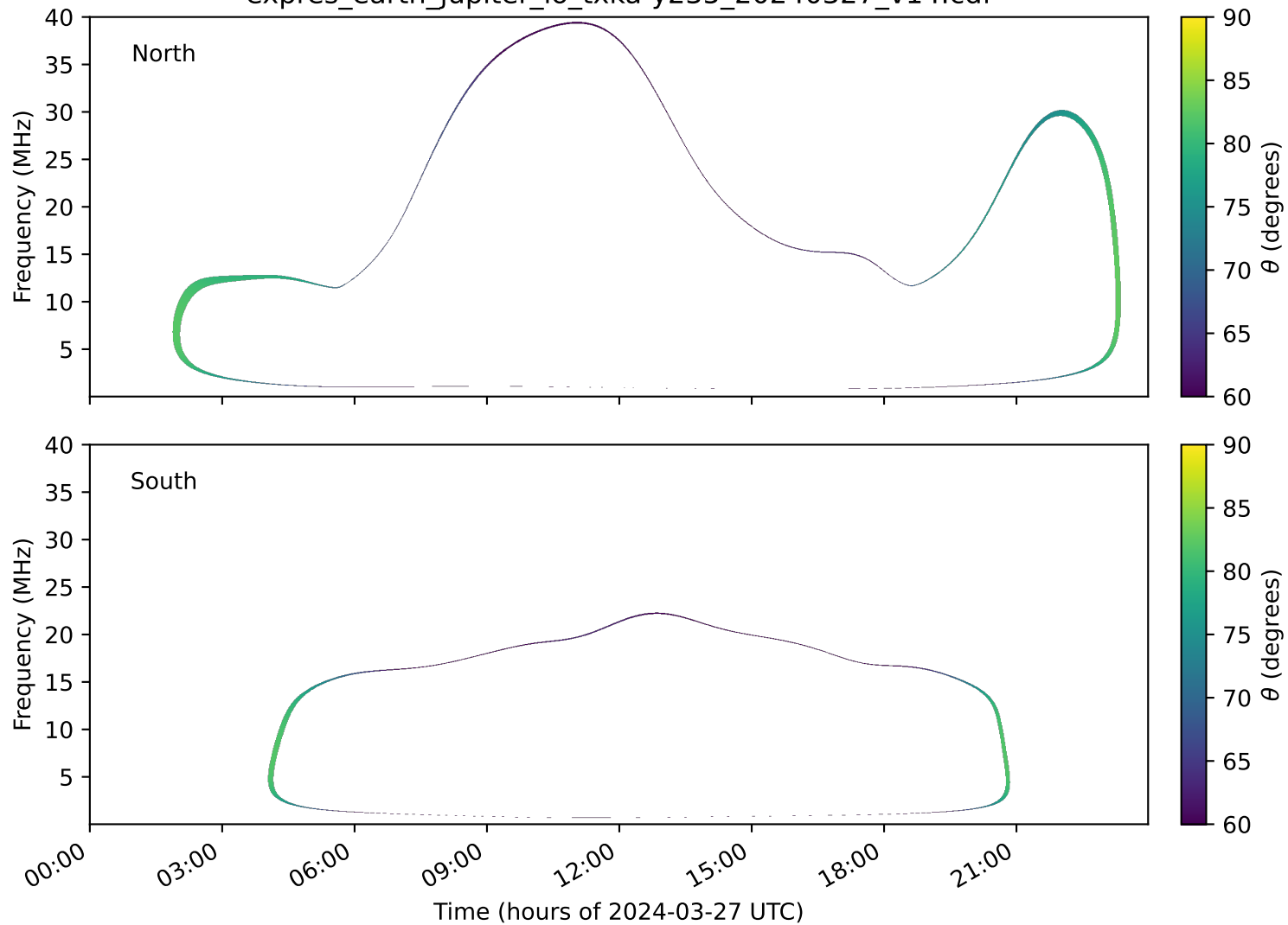
expres_earth_jupiter_io_txka-y235_20240327_v14.cdf
