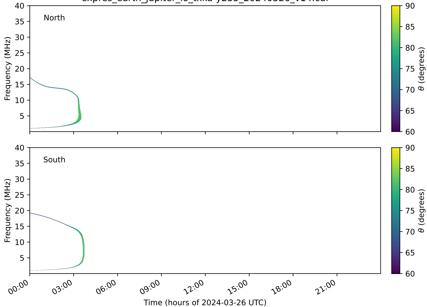
expres_earth_jupiter_io_txka-y235_20240326_v14.cdf
