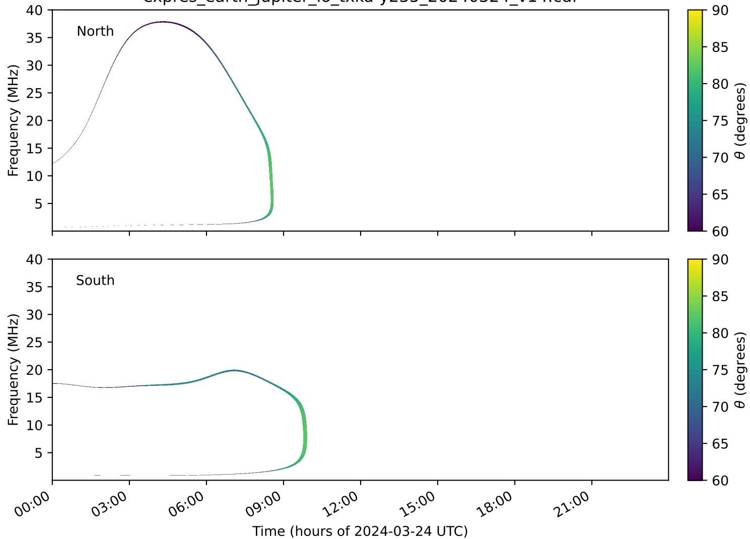
expres_earth_jupiter_io_txka-y235_20240324_v14.cdf
