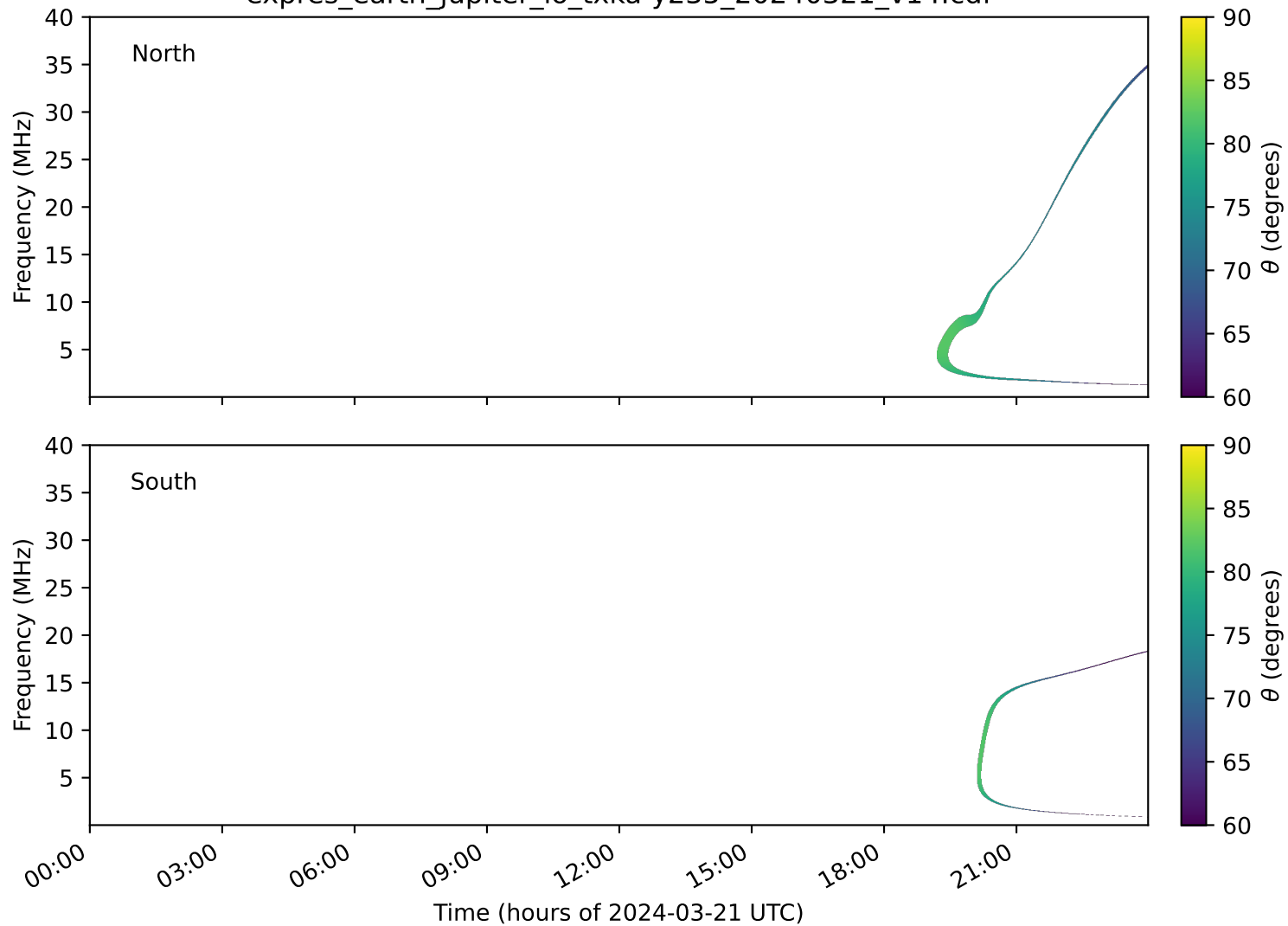
expres_earth_jupiter_io_txka-y235_20240321_v14.cdf
