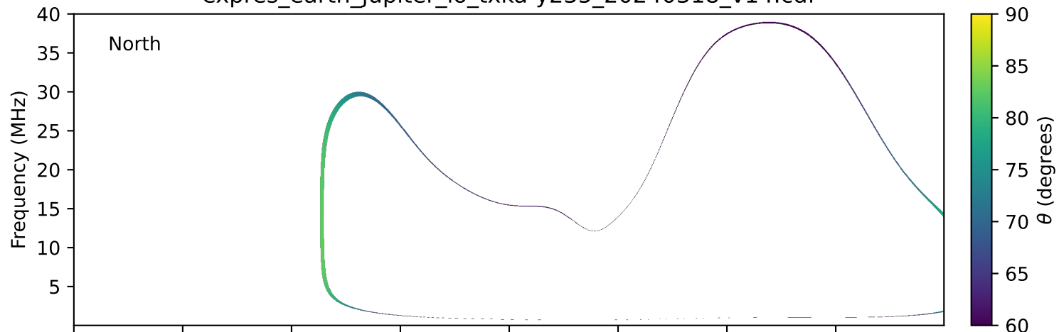
expres_earth_jupiter_io_txka-y235_20240318_v14.cdf
