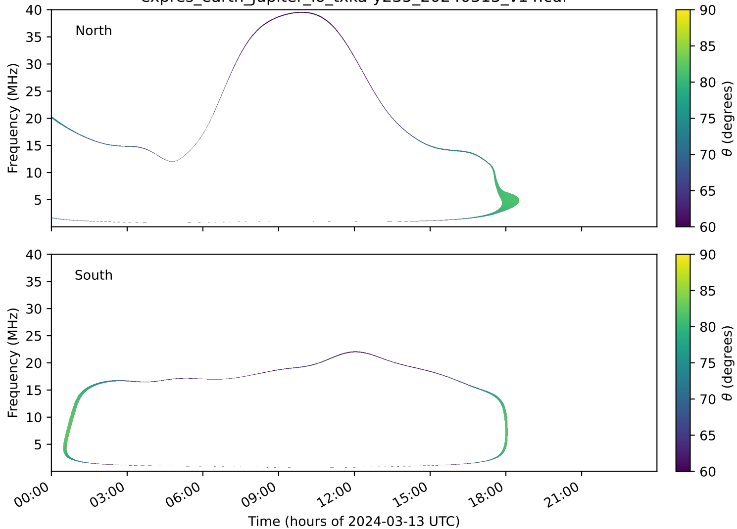
expres_earth_jupiter_io_txka-y235_20240313_v14.cdf
