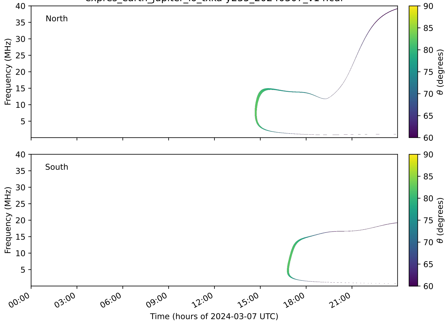
expres_earth_jupiter_io_txka-y235_20240307_v14.cdf
