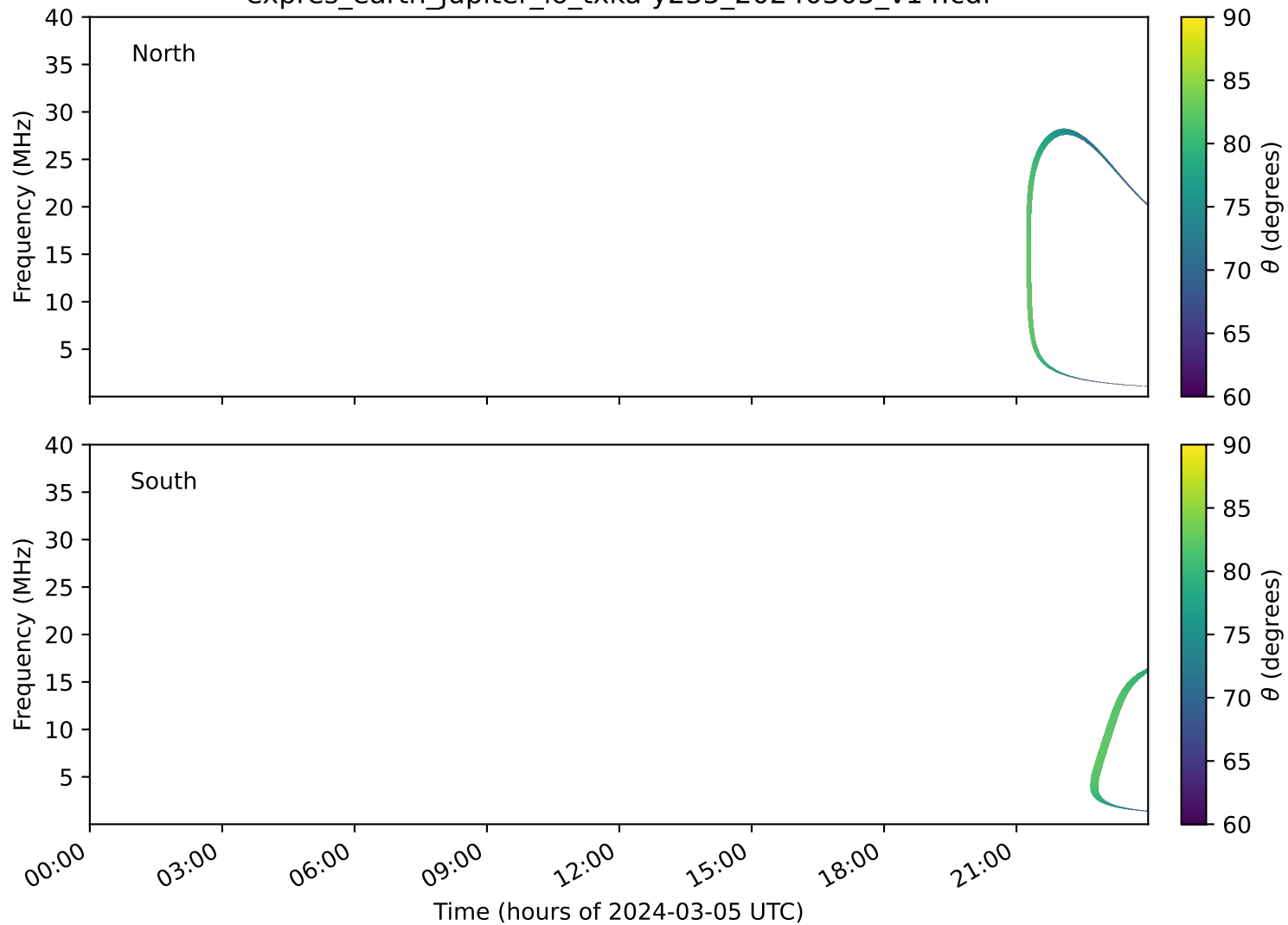
expres_earth_jupiter_io_txka-y235_20240305_v14.cdf
