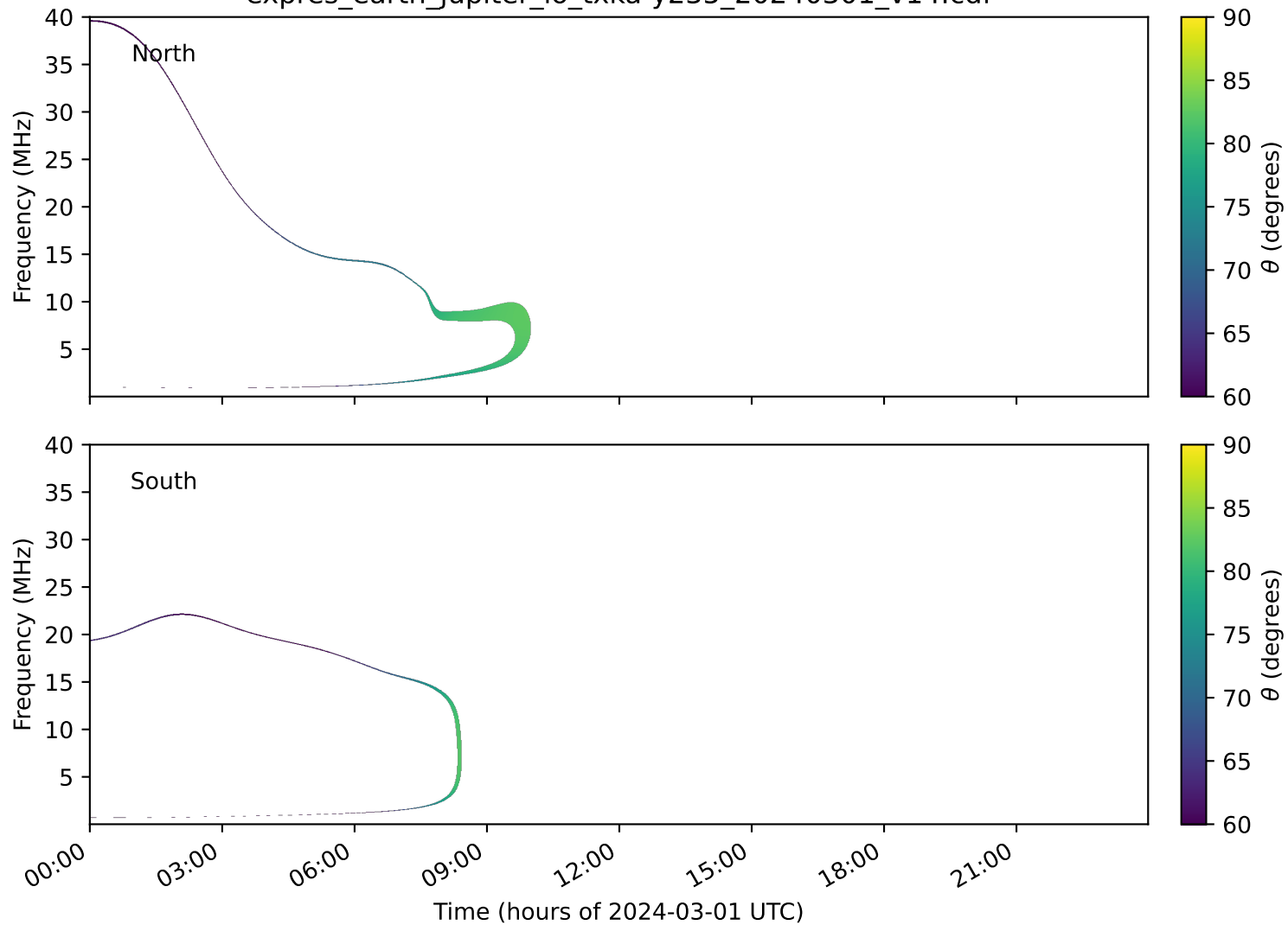
expres_earth_jupiter_io_txka-y235_20240301_v14.cdf
